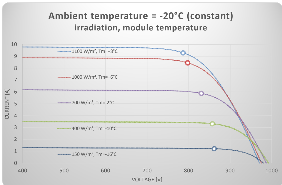
Figure 1: Characteristics T_a = -20\text{ °C} (source: internal analysis - Fronius International GmbH)
